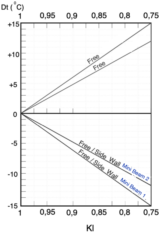
CORRECTION FACTOR FOR THROW (L0.2) DT (-).
