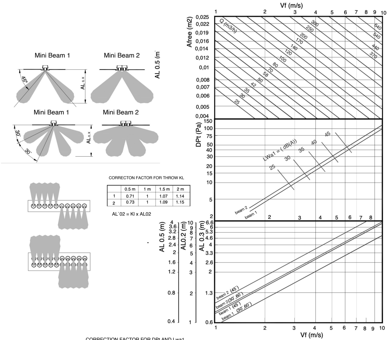
CORRECTION FACTOR FOR Dpt AND Lwa1.
