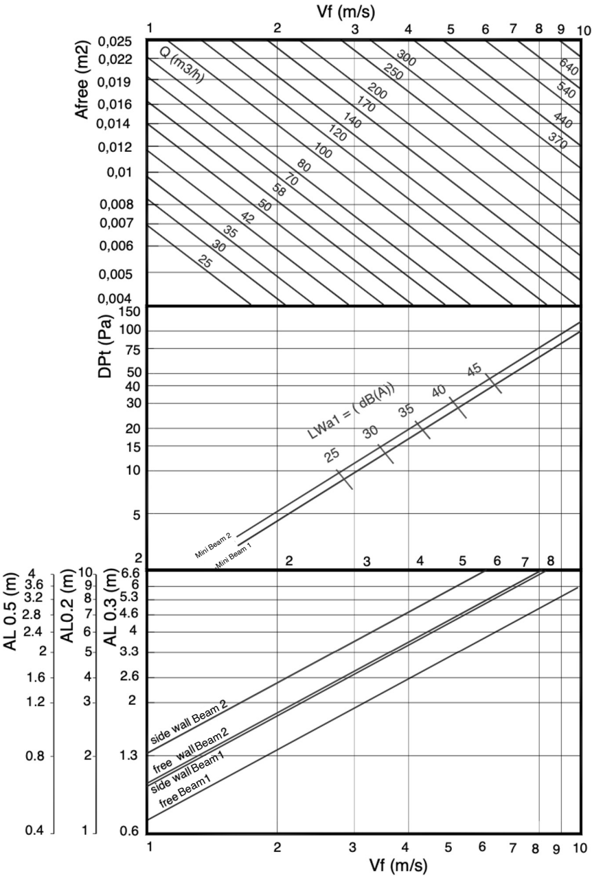
CORRECTION FACTOR FOR DPt AND Lwa1.
