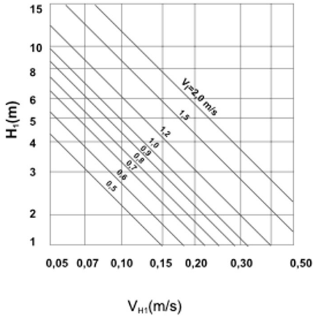
VELOCITY DIAGRAM
