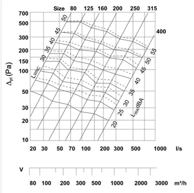
PRESSURE DROP AND SOUND LEVEL CURVE
