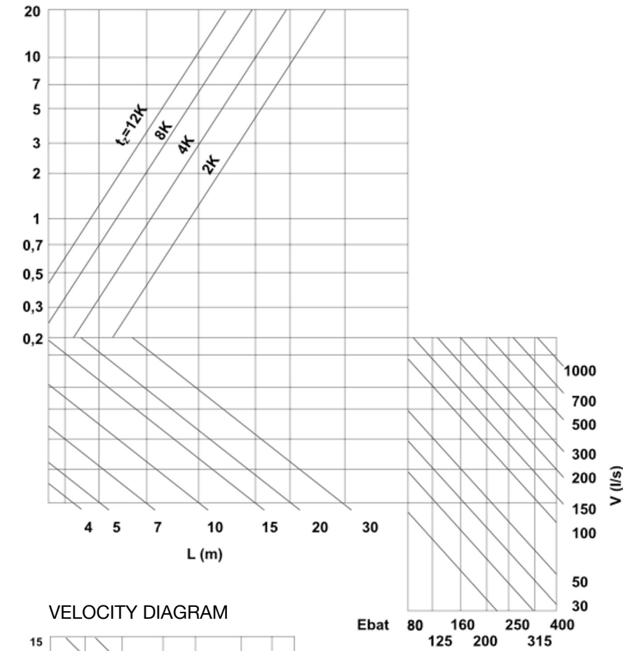
THROW LENGTH AND AIR STREAM DEVIATION
