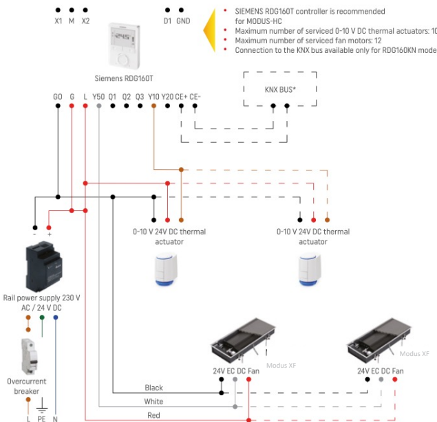
Configuration of RDG160T basic work parameters for MODUS-HC units
