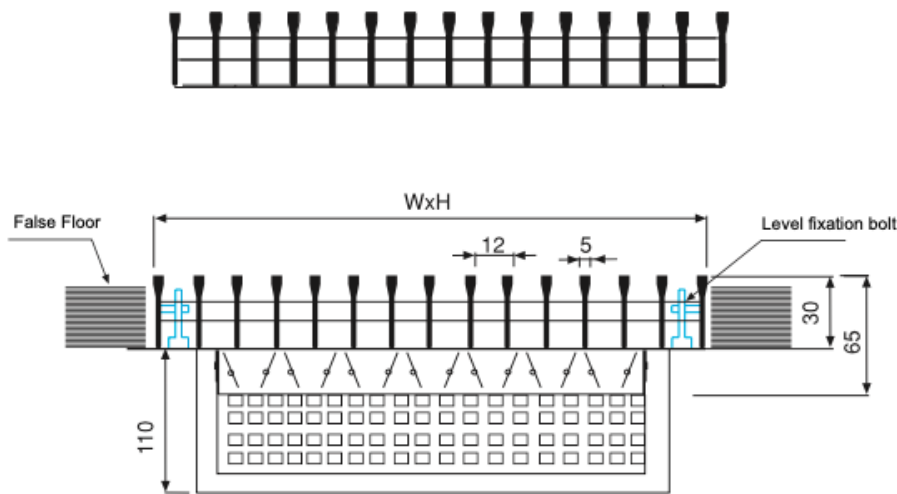
False Floor Linear Grille With Damper and Dust Collecting Casing
