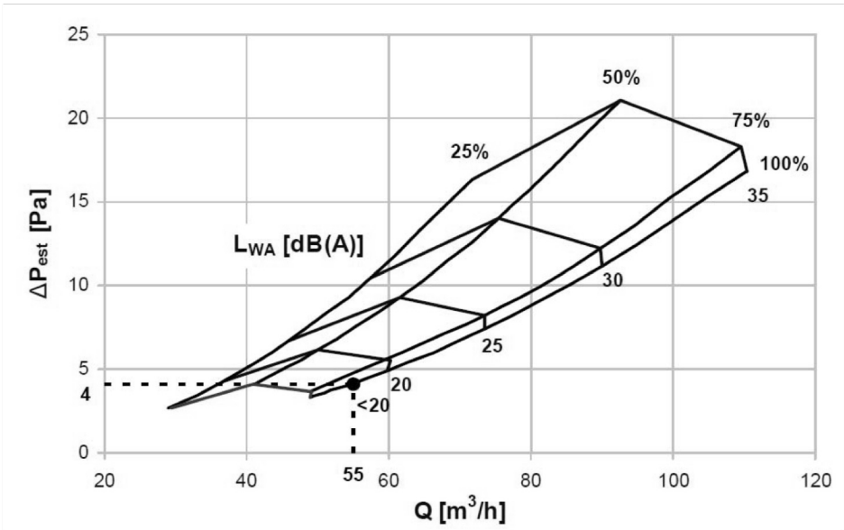
Size 200 (without plenum) Sound power % (Dirt trap opening percentage) Graph 2
