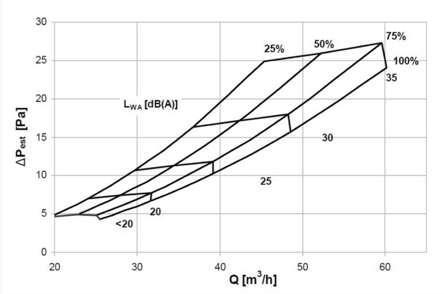
Size 200 (without plenum) Sound power % (Dirt trap opening percentage) Graph 2
