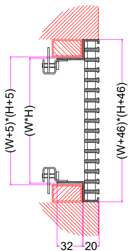
Clips ( Plate Spring Fixing )
